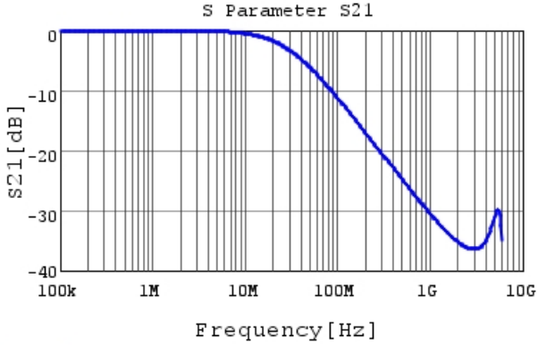
NFM18CC221R1C3 S21 DCOV,25degC, Feedthrough
