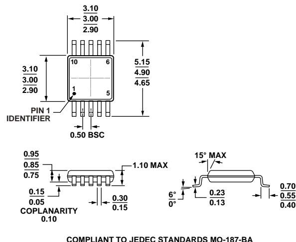
COMPLIANT TO JEDEC STANDARDS MO-187-BA Figure 95. 10-Lead Mini Small Outline Package [MSOP] (RM-10) Dimensions shown in millimeters
