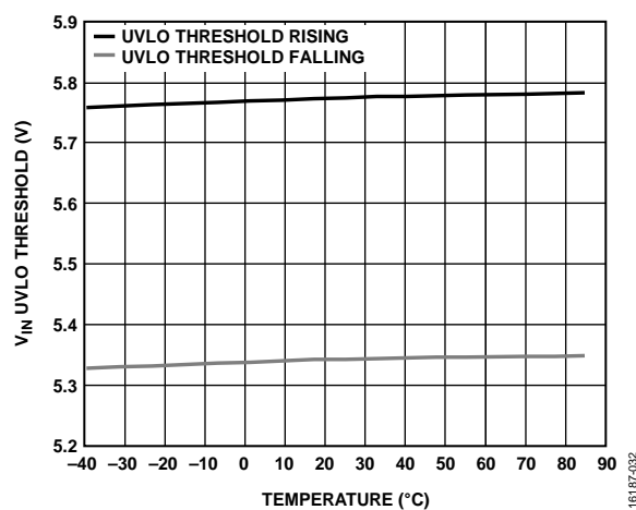
Figure 32. Input Voltage ( V_{IN} ) UVLO Threshold vs. Temperature
