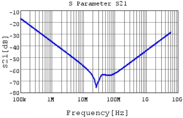
NFM21PC474R1C3 S21 DCOV,25degC, Feedthrough
