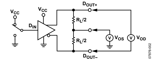
Figure 2. Test Circuit for Driver V_{OD} and V_{OS}
