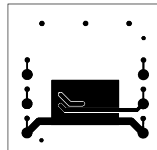
Solder Side
