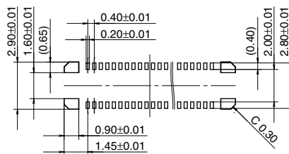
Recommended metal mask pattern Metal mask thickness: When 120μm (Terminal opening ratio: 70%) (Metal-part opening ratio: 70%)
