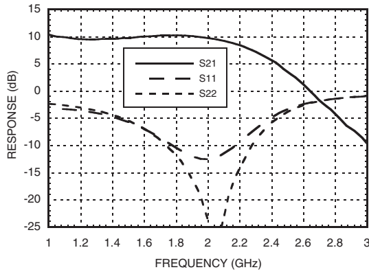
Broadband Gain & Return Loss @ 2100 MHz
