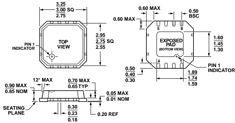
Figure 44. 8-Lead Frame Chip Scale Package [LFCS_VD] 3 mm x 3 mm Body, Very Thin, Dual Lead (CP-8-2)
