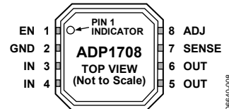
Figure 9. 8-Lead LFCSP, ADP1708
