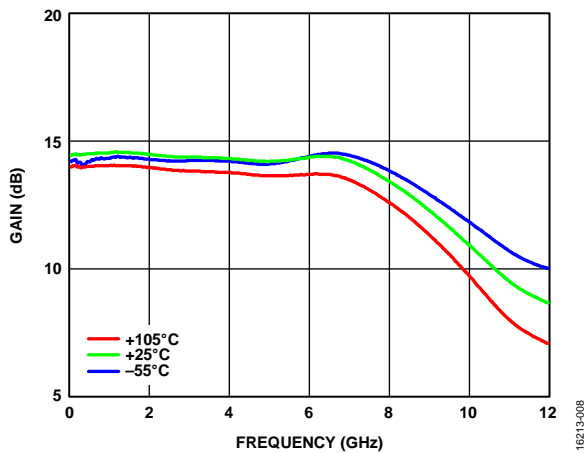
Figure 8. Gain vs. Frequency at Various Temperatures
