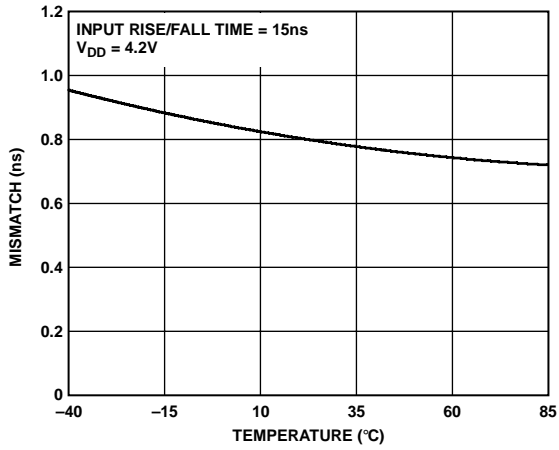
Figure 23. Rise-Time-to-Fall-Time Mismatch vs. Temperature
