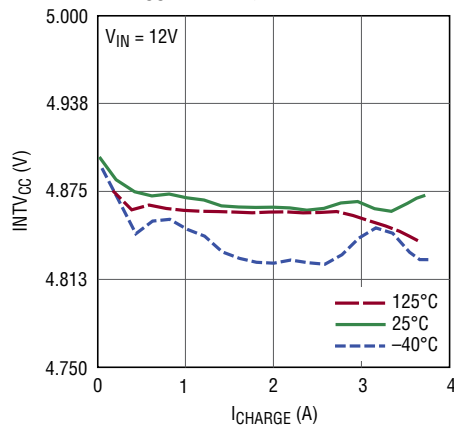
INTV CC vs Charge Current
