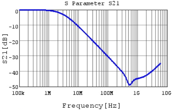
NFM21CC222R1H3 S21 DCOV,25degC, Feedthrough
