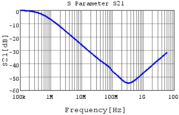
NFM15CC223C1C3 S21 DCOV,25degC, Feedthrough
