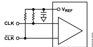
Figure 32. Use of V_{REF} to Provide Low Impedance Termination into V_S/2
