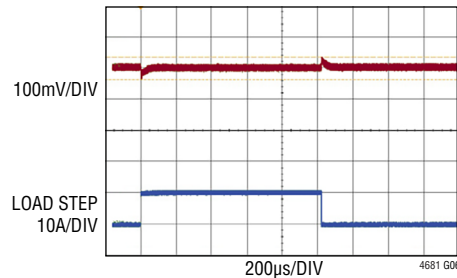
Single Channel Load Transient Response (10A) to (20A) Load Step, 10\text{A}/\mu\text{s} 12\text{V}_{\text{IN}} to 1.2\text{V}_{\text{OUT}} , f_{\text{SW}} = 350\text{kHz}
