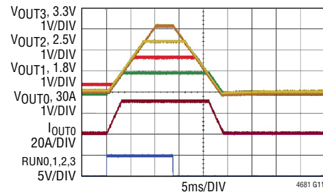
FIGURE 48 CIRCUIT, 12\text{V}_{\text{IN}} , 30\text{A} ON V_{\text{OUT0}} NO LOAD ON OTHER OUTPUTS AND 0.5\text{V} PREBIAS ON V_{\text{OUT1}}
