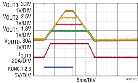
FIGURE 48 CIRCUIT, 12\text{V}_{\text{IN}} , 30\text{A} ON V_{\text{OUT0}} NO LOAD ON OTHER OUTPUTS
