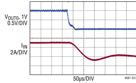
FIGURE 48 CIRCUIT, 12\text{V}_{\text{IN}} , 30\text{A} LOAD ON V_{\text{OUT0}} PRIOR TO APPLICATION OF SHORT-CIRCUIT USE HIGH RANGE OF I LIMIT SYSTEM SHORT-CIRCUIT USING LOW IMPEDANCE COPPER ACROSS OUTPUT (HARD SHORT)
