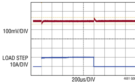
Single Channel Load Transient Response (10A) to (20A) Load Step, 10\text{A}/\mu\text{s} 12\text{V}_{\text{IN}} to 2.5\text{V}_{\text{OUT}} , f_{\text{SW}} = 500\text{kHz}
