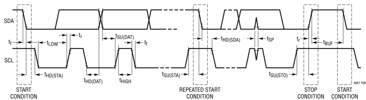
Figure 6. PMBus Timing Diagram
