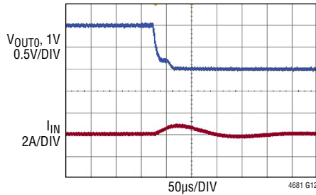
FIGURE 48 CIRCUIT, 12\text{V}_{\text{IN}} , NO LOAD ON V_{\text{OUT0}} PRIOR TO APPLICATION OF SHORT-CIRCUIT USE HIGH RANGE OF I LIMIT SYSTEM SHORT-CIRCUIT USING LOW IMPEDANCE COPPER ACROSS OUTPUT (HARD SHORT)
