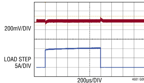
Single Channel Load Transient Response (10A) to (20A) Load Step, 10\text{A}/\mu\text{s} 12\text{V}_{\text{IN}} to 3.3\text{V}_{\text{OUT}} , f_{\text{SW}} = 500\text{kHz}
