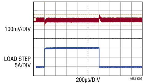
Single Channel Load Transient Response (10A) to (20A) Load Step, 10\text{A}/\mu\text{s} 12\text{V}_{\text{IN}} to 1.5\text{V}_{\text{OUT}} , f_{\text{SW}} = 350\text{kHz}
