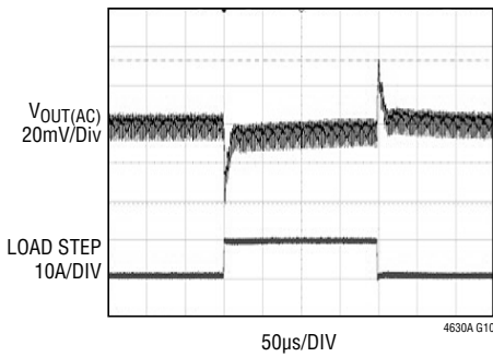
3.3V Dual Phase Single Output Load Transient Response
