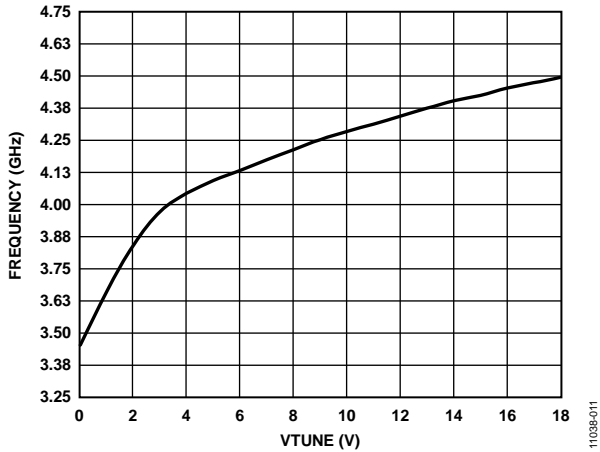
Figure 11. RFOUT/2 Frequency vs. Tuning Voltage
