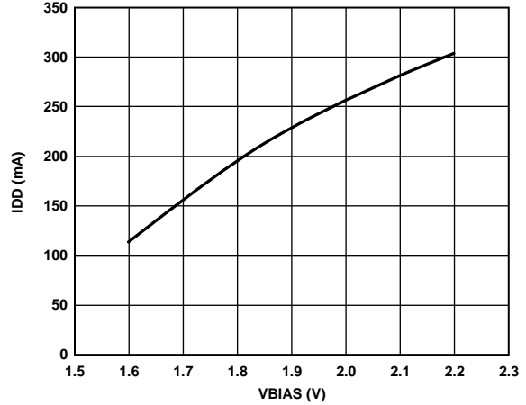
Figure 16. IDD vs. VBIAS with VTUNE = 6 V
