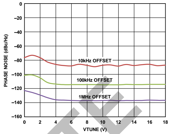
Figure 8. Phase Noise vs. Tuning Voltage
