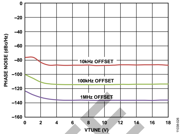
Figure 20. Phase Noise vs. Tuning Voltage with VDD = 3V
