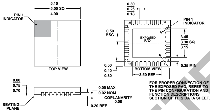
Figure 23. 32-Lead Lead Frame Chip Scale Package [LFCSP_WQ] 5 mm × 5 mm Body, Very Very Thin Quad (CP-32-13) Dimensions shown in millimeters
