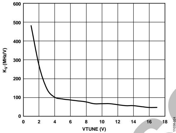
Figure 18. Sensitivity vs. Tuning Voltage with VDD = 3V
