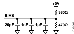
Figure 3. Bias Network for 5 V Operation
