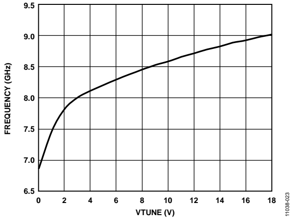
Figure 17. Frequency vs. Tuning Voltage with VDD = 3V
