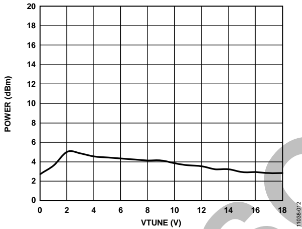
Figure 12. RFOUT/2 Output Power vs. Tuning Voltage
