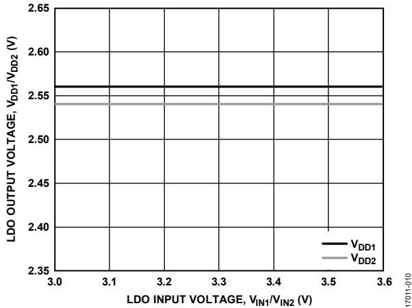
Figure 15. LDO Output Voltage, V_{\text{DD1}}/V_{\text{DD2}} vs. LDO Input Voltage, V_{\text{IN1}}/V_{\text{IN2}}
