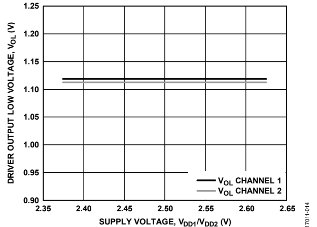
Figure 19. Driver Output Low Voltage, V_{\text{OL}} vs. Supply Voltage, V_{\text{DD1}}/V_{\text{DD2}}
