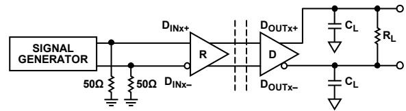
Figure 39. Timing Test Circuit
