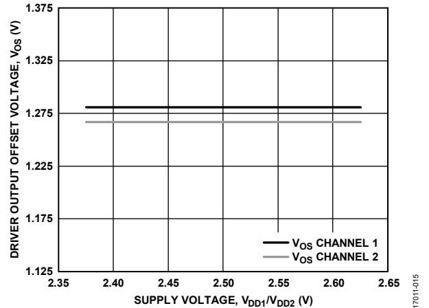
Figure 20. Driver Output Offset Voltage, V_{\text{OS}} vs. Supply Voltage, V_{\text{DD1}}/V_{\text{DD2}}
