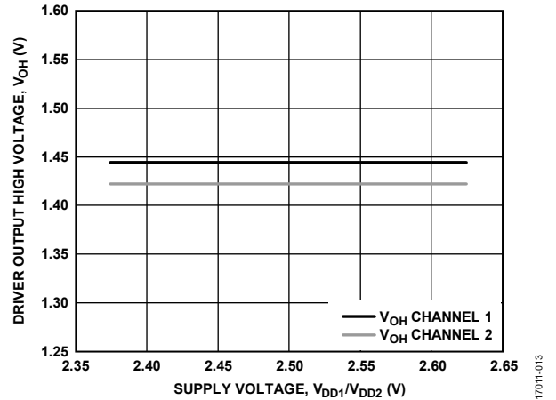
Figure 18. Driver Output High Voltage, V_{\text{OH}} vs. Supply Voltage, V_{\text{DD1}}/V_{\text{DD2}}
