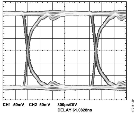
Figure 35. Eye Diagram for D_{OUT2\pm} at 300 MHz
