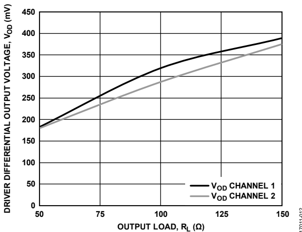
Figure 17. Driver Differential Output Voltage, V_{\text{OD}} vs. Output Load, R_{\text{L}}
