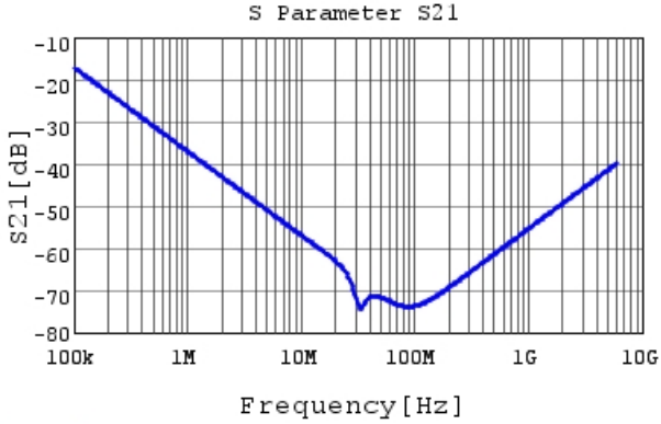
■ NFM18PS474R0J3 S21 DCOV,25degC, Feedthrough
