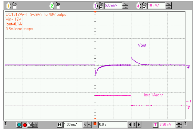
Figure 5. Fast transient response of DC1317A-H is superior to many competing power modules without the additional output capacitors.
