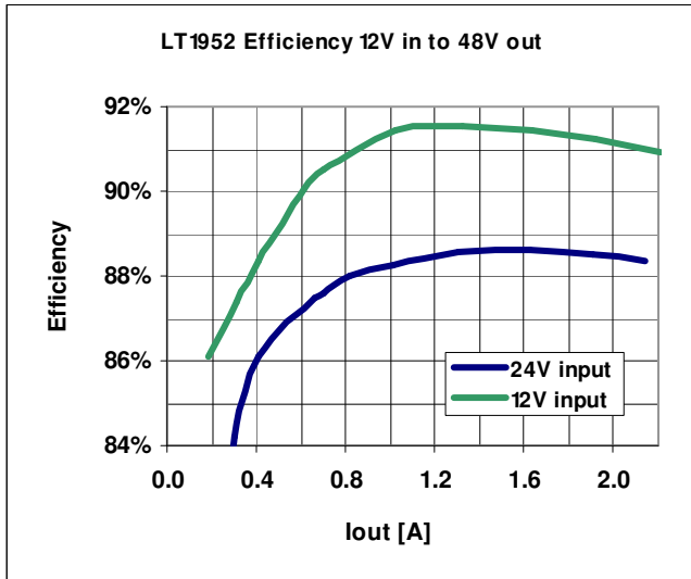
Figure 3. High efficiency of DC1317A-H allows the board to be used in thermally critical applications. Up to 2A of output current can be drawn with proper air flow.
