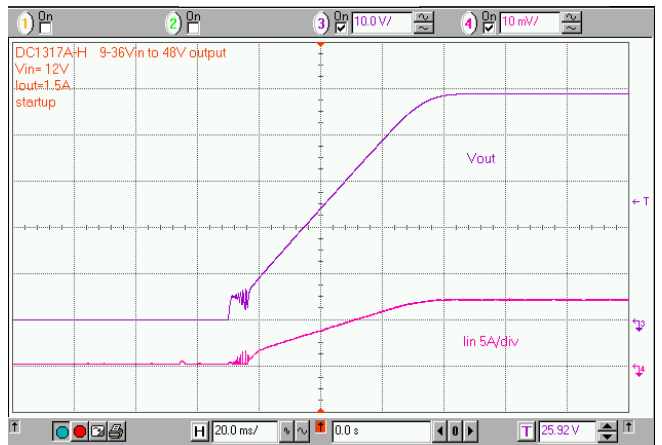
Figure 6. The LT4430 opto coupler driver produces monotonic output voltage rise at startup without output voltage overshoot.
