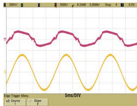
Figure 6. 230VAC (PF = 0.97)
