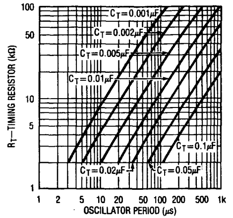
Oscillator Period
