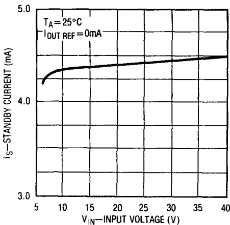
Standby Current
