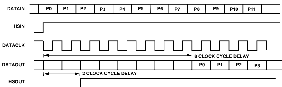
Figure 14. 4:4:4 Timing Mode
