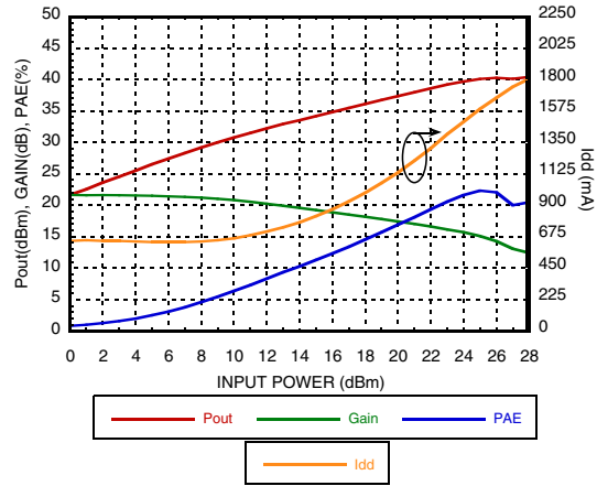
Power Compression @ 18 GHz
