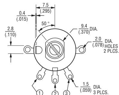
SHAFT SHOWN IN CCW POSITION
