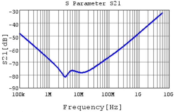
NFM31PC276B0J3 S21 DCOV,25degC, Feedthrough
