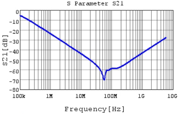
NFM21PC104R1E3 S21 DCOV,25degC, Feedthrough
