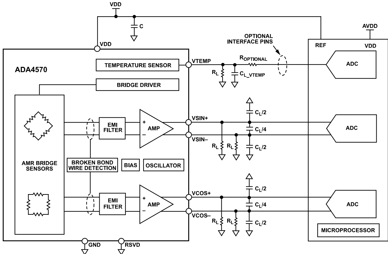
Figure 18. Typical Application Diagram
