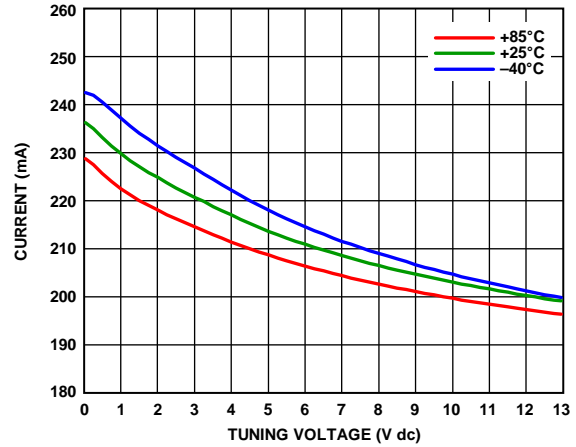
Figure 11. Supply Current ( I_{CC} ) vs. Tuning Voltage
