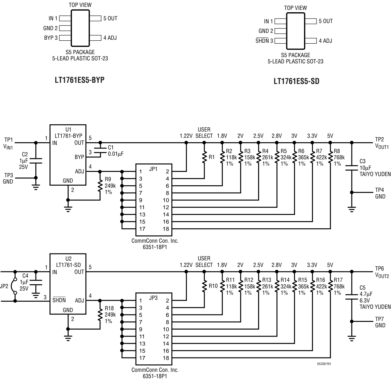
Figure 1. 100mA Low Noise LDO Regulator
