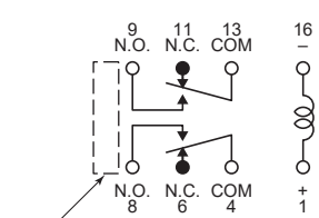
Schematic (Bottom view)
