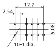
Recommended PC board pattern (BOTTOM VIEW)
