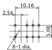
Recommended PC board pattern (BOTTOM VIEW)
