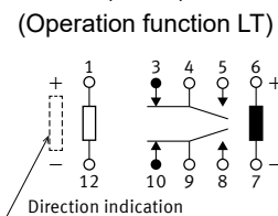
Schematic (BOTTOM VIEW) (Reset)
