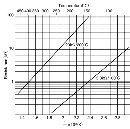
Resistance-temperature characteristics (Fig.1)
