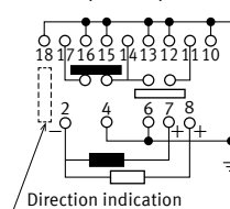
2 coil latching (Reset)
