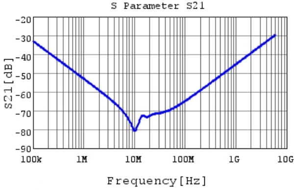
NFM21PC475B1A3 S21 DCOV,25degC, Feedthrough
