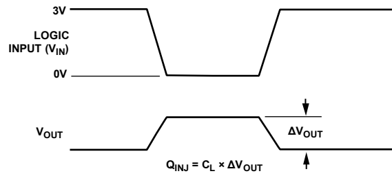
Figure 28. Charge Injection
