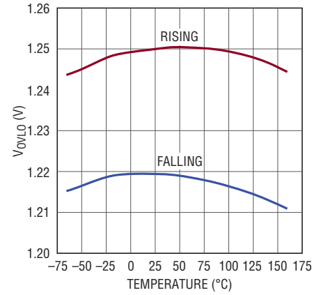
OVLO Threshold Voltage vs Temperature
