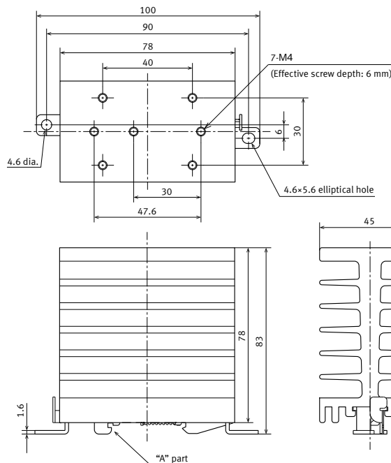
External dimensions
