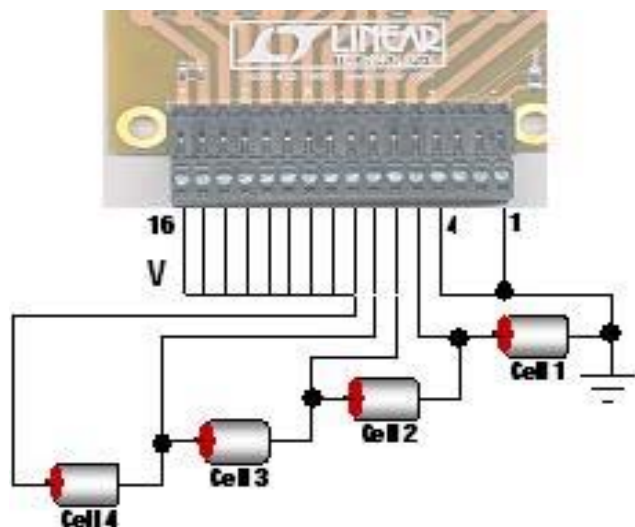
Figure 1. Connection of four cells (cell voltages at least 2.5V)
