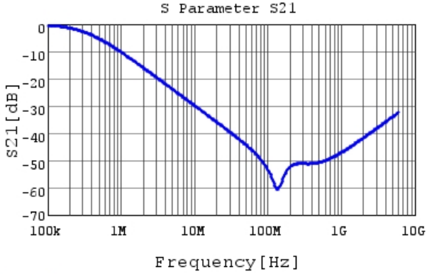
NFM21CC223R1H3 S21 DCOV,25degC, Feedthrough
