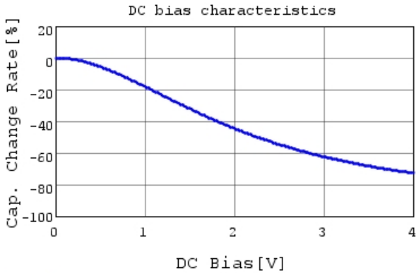
NFM15PC435R0G3 C-DC bias capchange, 25.0degC
