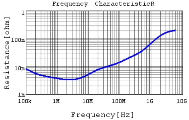
NFM15PC435R0G3 R DCOV,25degC, Non-feedthro
