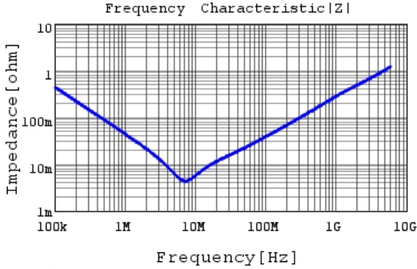
NFM15PC435R0G3 |Z| DCOV,25degC, Non-feedthro
