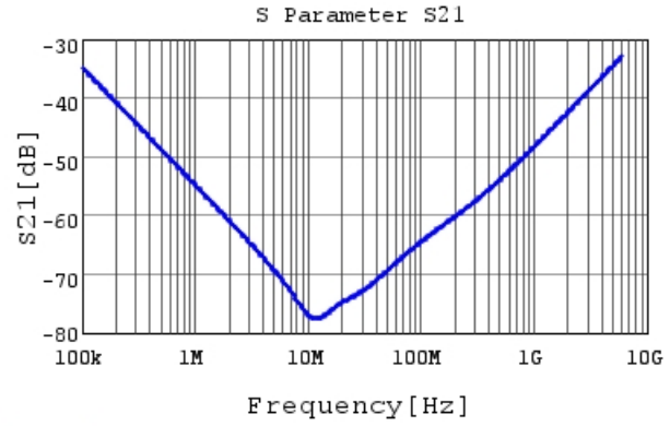
■ NFM15PC435R0G3 S21 DCOV, 25degC, Feedthrough
