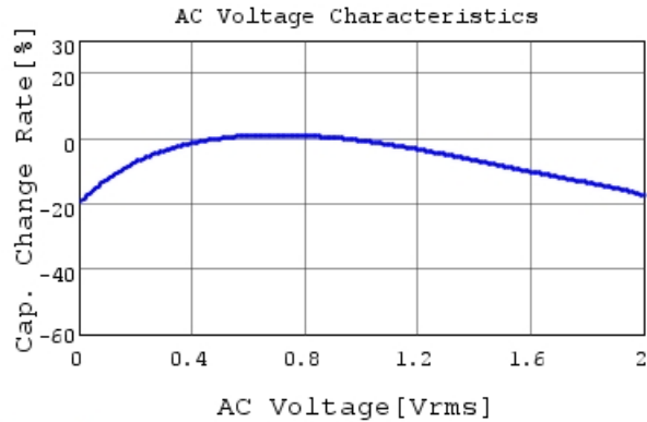
NFM15PC435R0G3 C-AC Voltage capchange, DCOV,
