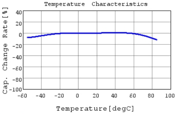
■ NFM15PC435R0G3 C-Temp. capchange, DCOV, ACO.
