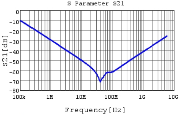
NFM21PC224R1C3 S21 DCOV,25degC, Feedthrough
