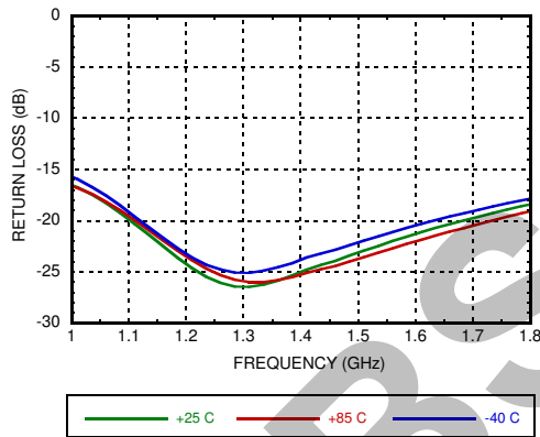
Input Return Loss vs. Temperature [1]
