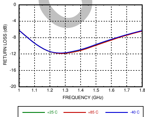
Output Return Loss vs. Temperature [1]
