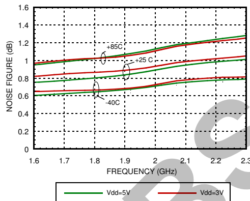
Noise Figure vs. Temperature [1] [2] [3]
