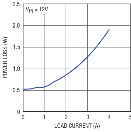
Figure 9. 5V Loss
