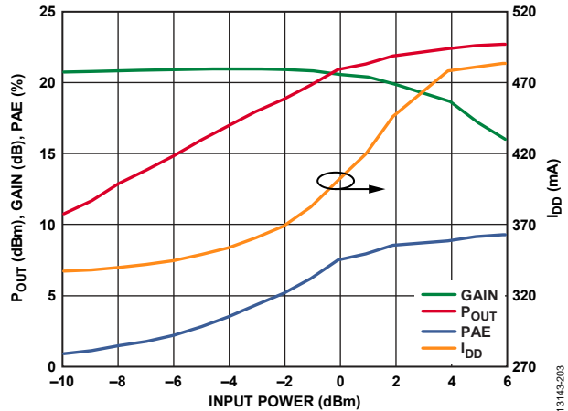
Figure 31. P_{OUT} , Gain, PAE, and I_{DD} vs. Input Power at 65 GHz
