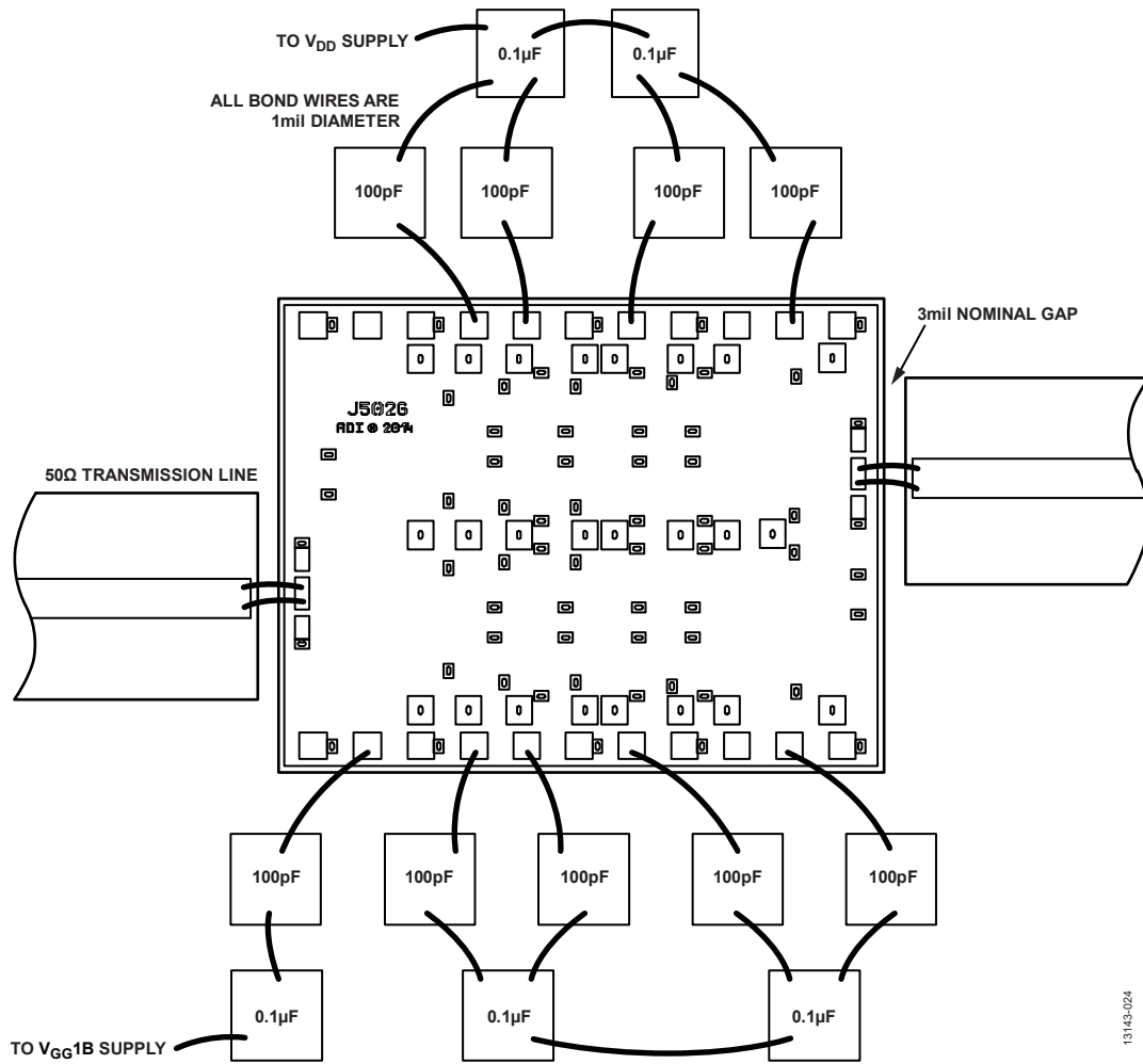
Figure 40. Assembly Diagram
