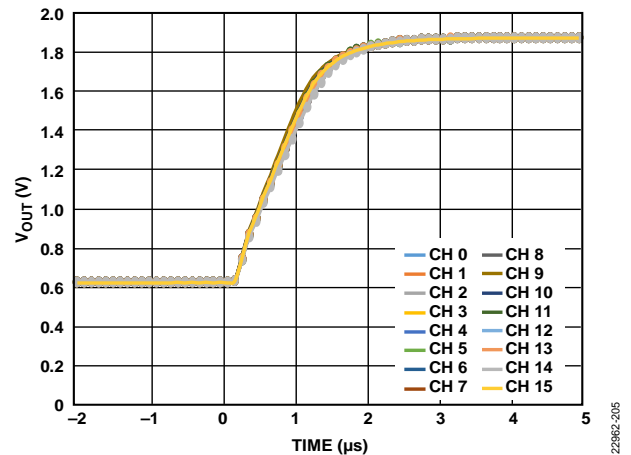
Figure 40. Settling Time
