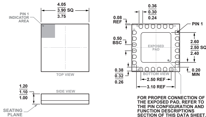
24-Terminal Ceramic Leadless Chip Carrier [LCC] (E-24-2)
