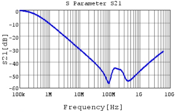
NFM31HK223R1H3 S21 DCOV,25degC, Feedthrough
