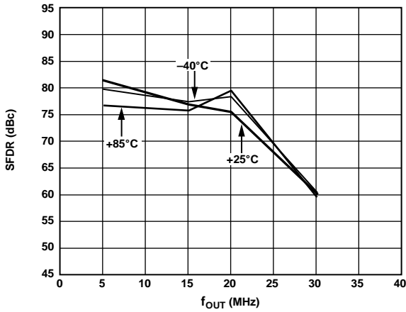
Figure 40. SFDR vs. Temperature at 80 MSPS
