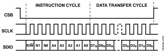
Figure 72. Serial Register Interface Timing, MSB First Write
