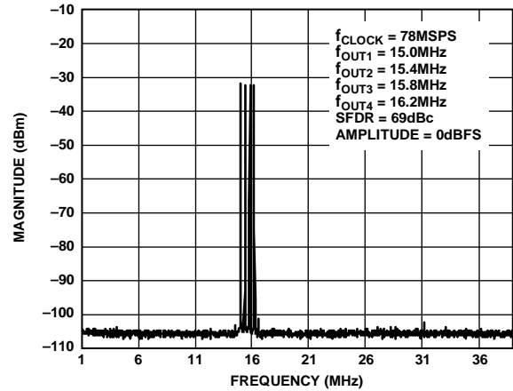
Figure 43. Four-Tone SFDR
