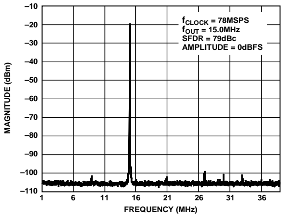
Figure 41. Single-Tone SFDR
