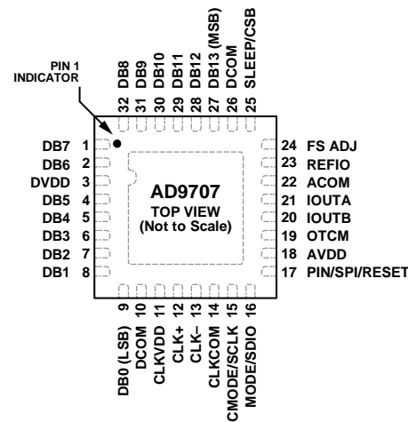
Figure 3. AD9707 Pin Configuration
